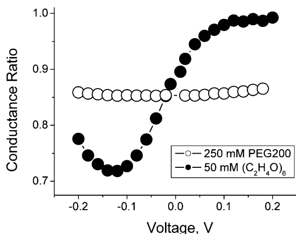
FIGURE 1 Comparison of the effects of the crown ether ( \text{C}_2\text{H}_4\text{O} ) 6 (●) and poly(ethylene glycol) (PEG) with molecular weight of 200 (○) on the conductance of a single \alpha -hemolysin channel reconstituted in a planar bilayer. Both the crown and PEG were added symmetrically to 1 M KCl solutions on both sides of the membrane. In both cases conductance is normalized to its value in pure salt solution. To facilitate the comparison, PEG was applied in a fivefold higher concentration than the crown.
